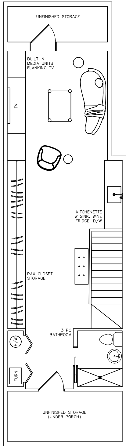
Potential Layout For Future Basement Renovation.
