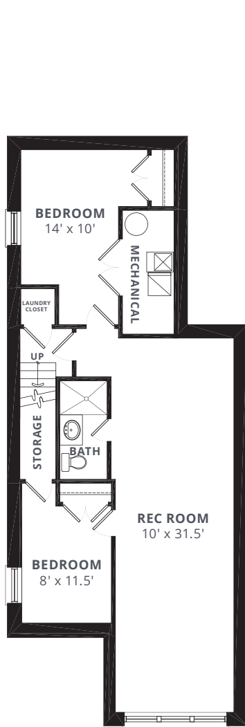
BASEMENT 810 Square Feet
